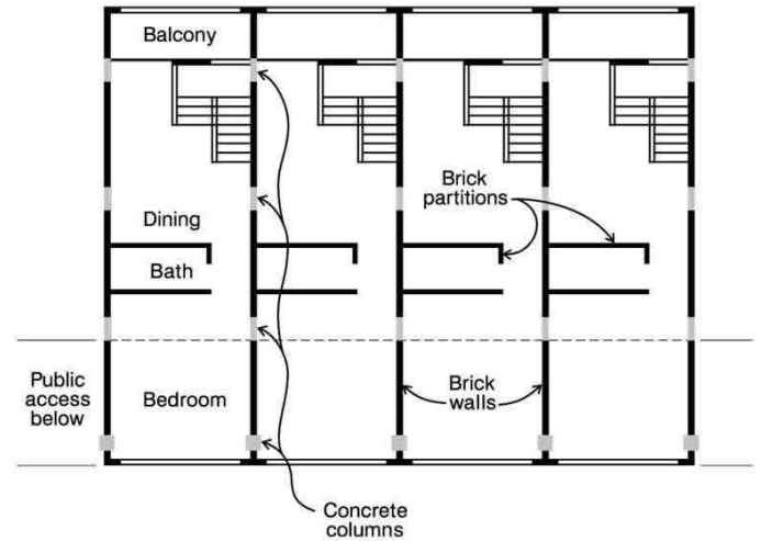
Typical Floor Plan -Past Practice (Source: EERI 2001)
