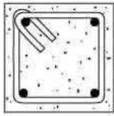
135° hooks
