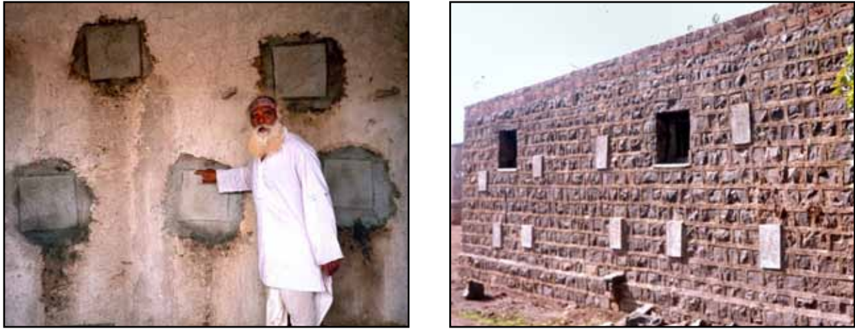
Figure 4.20: Examples of completed through-stone retrofit projects in Maharashtra, India (photos: S. Brzev)
