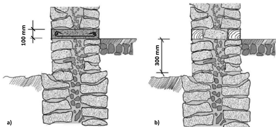
Figure 3.38 Stone masonry foundation with plinth bands: a) RC band, and b) timber band
